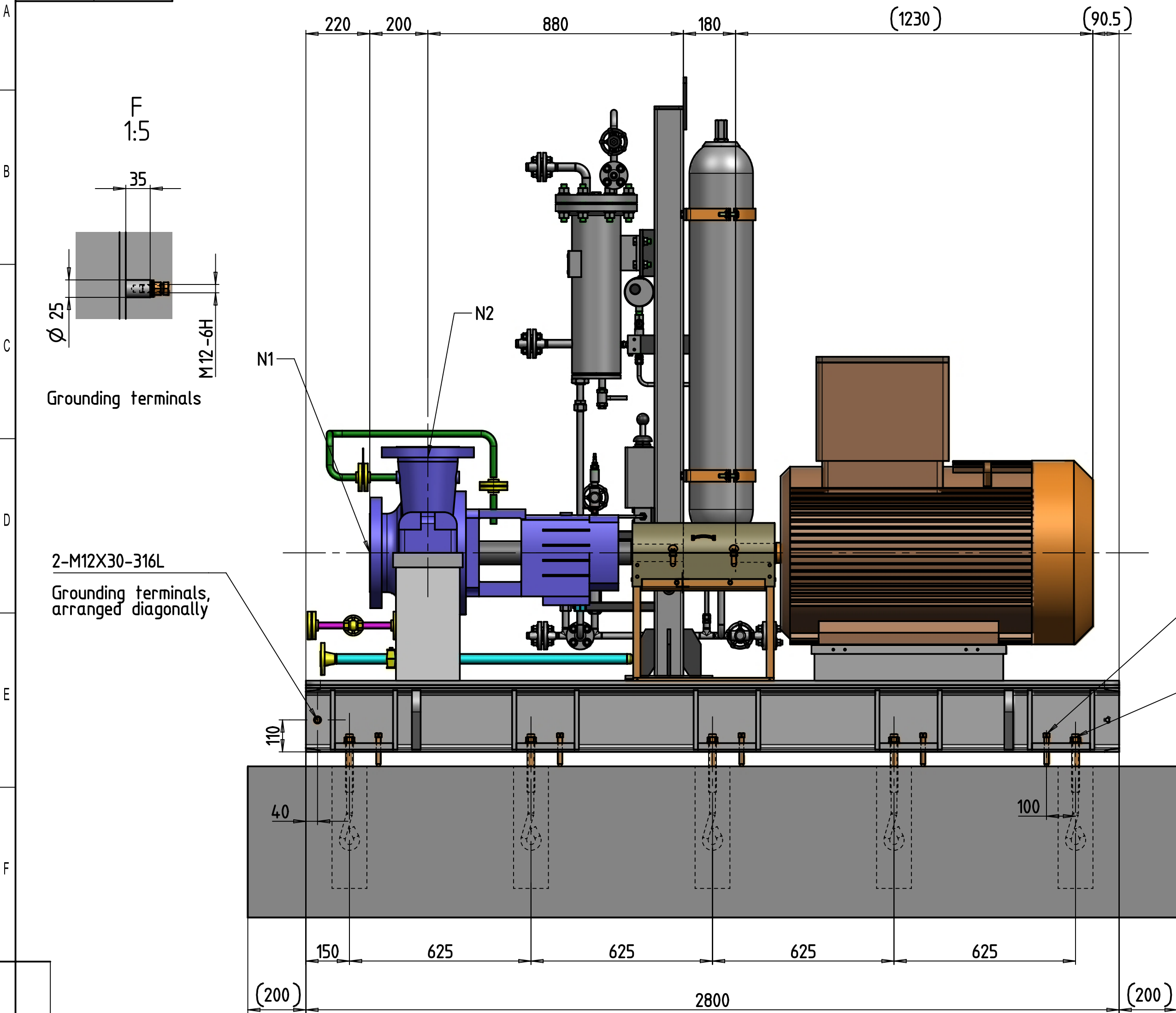
ELEVATION VIEW
