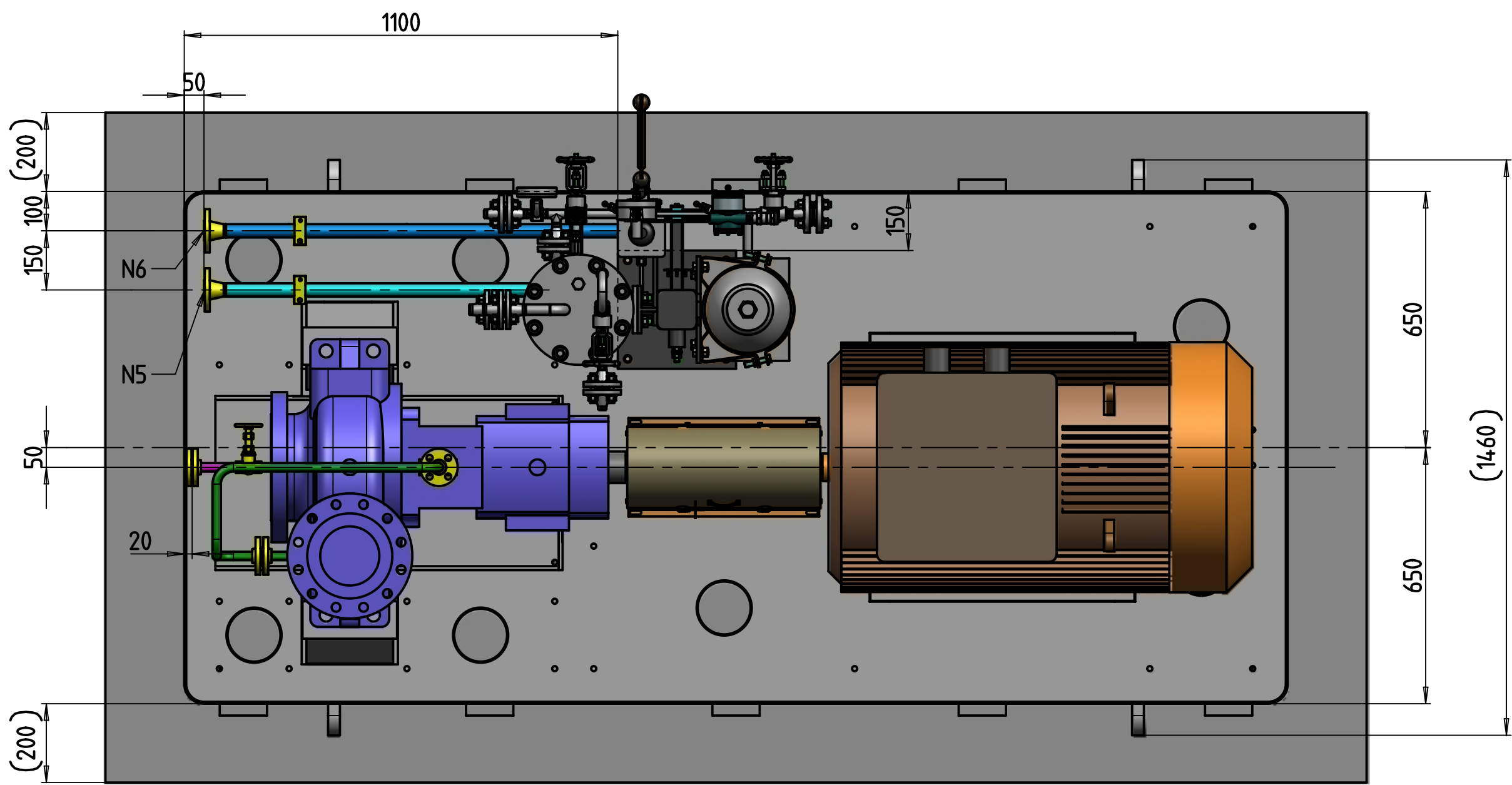
PLAN VIEW
