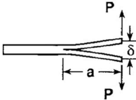
Figure 4.8: Schematic of the DCB test [49].
