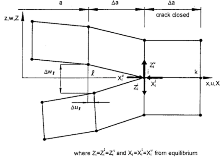
Figure 2.5: Virtual Crack Closure Technique (One-step crack closure technique) [17].
