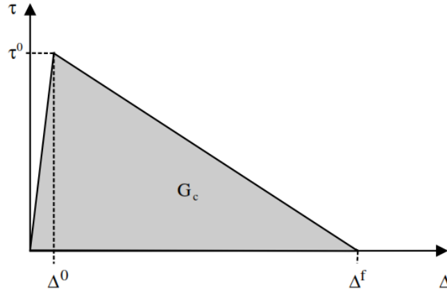
Figure 2.6: Bi-linear TSL as proposed by Turon et al. [12].
