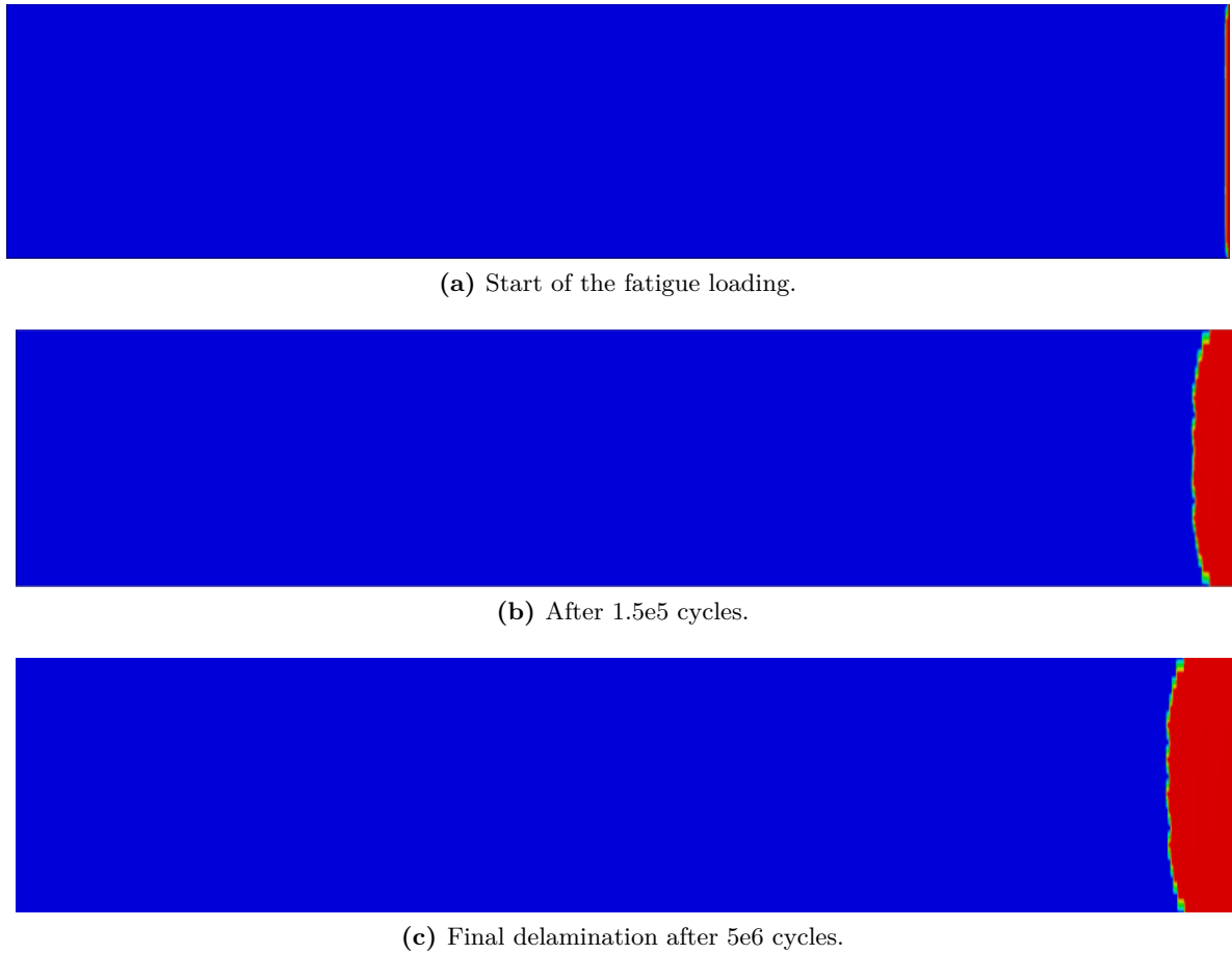
Figure 6.10: Delamination length at different stages during the fatigue analysis of the DCB specimen.
