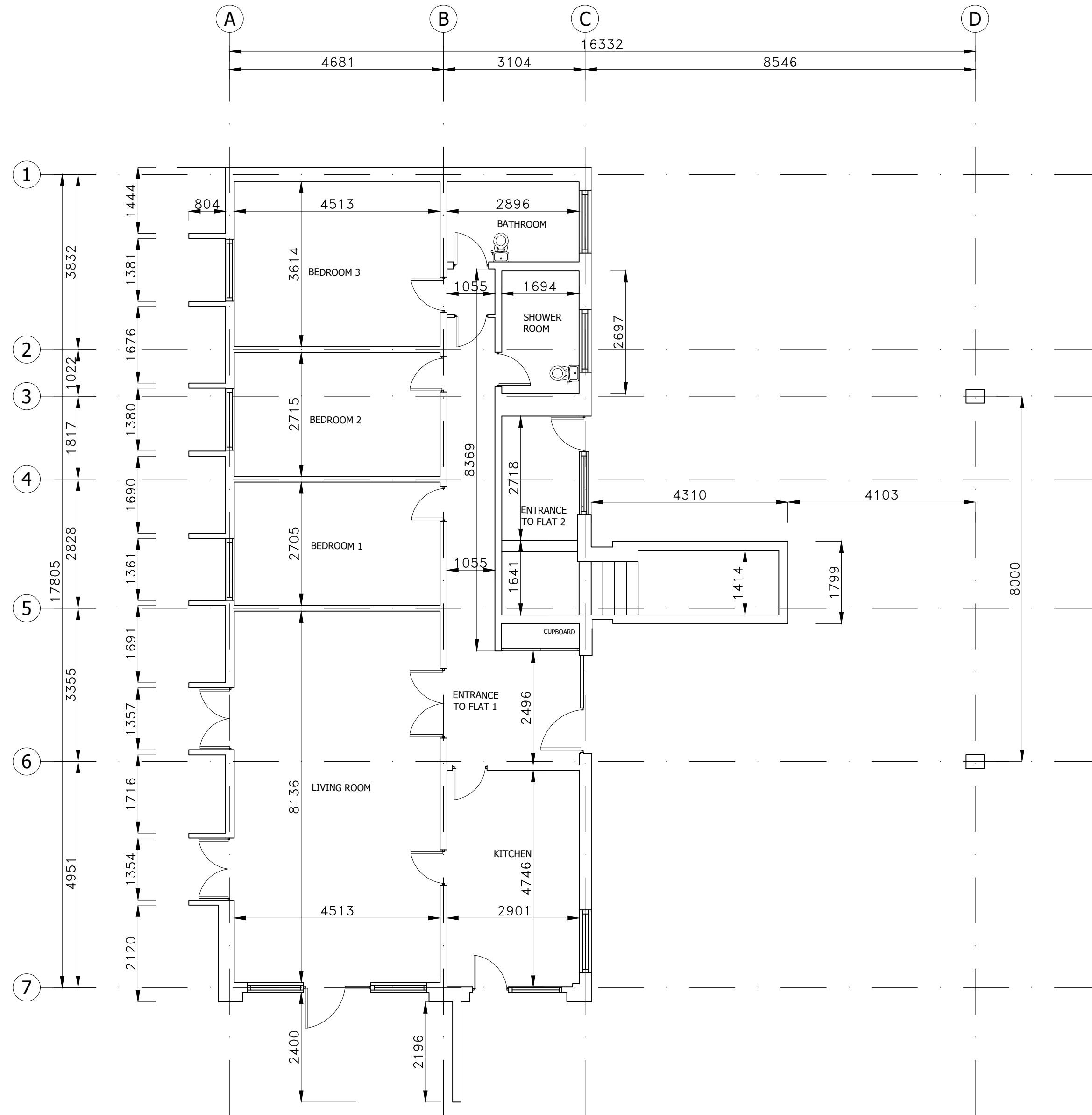
GROUND FLOOR 1:100
