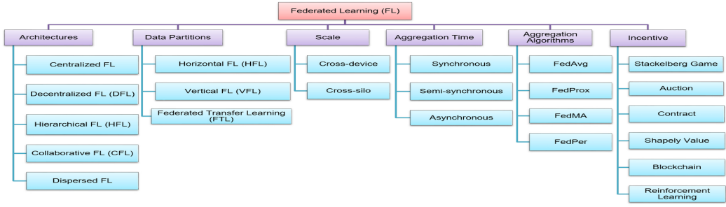
Fig. 1. FL taxonomy.
