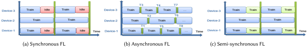
Fig. 2. FL synchronisation. (a) The synchronous FL scheme where T1 and T2 represent the synchronization points at which the devices can communicate with the FL coordinator. (b) The asynchronous FL scheme where each device can communicate with the FL whenever it has finished local training. (c) The semi-synchronous FL scheme where T1 and T2 represent the synchronization points at which the devices can communicate with the FL coordinator, and there is no idle time as in the synchronous scheme.
