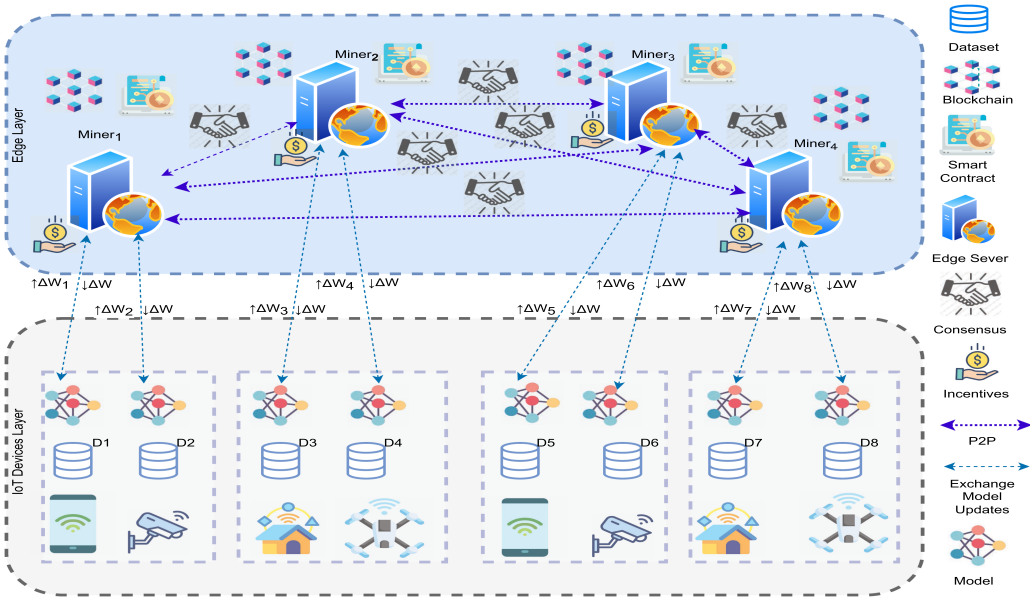
Fig. 8. The architecture for blockchain-enabled FL.
