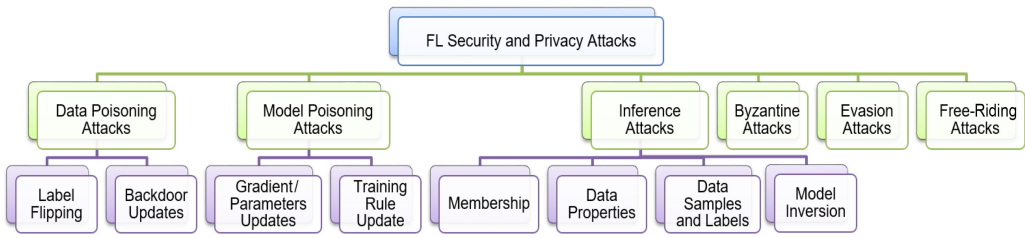
Fig. 3. FL security and privacy concerns.
