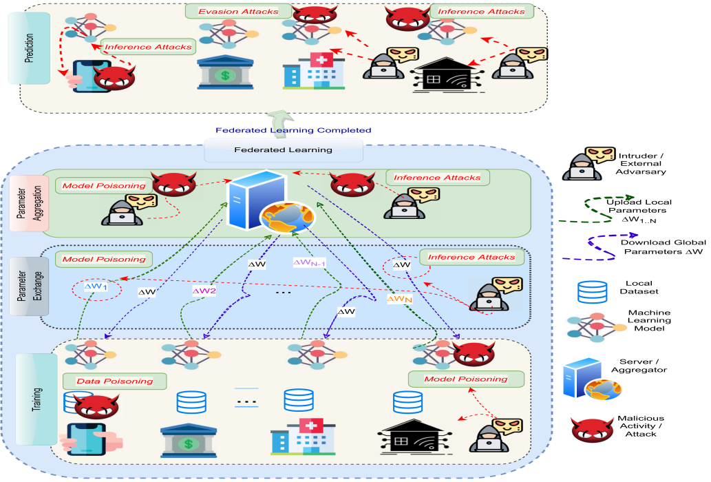
Fig. 4. FL threat model.
