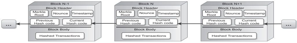
Fig. 6. Structure of a block in the blockchain.
