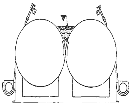
Figure 33. Atmospheric double-drum drier with center feed.
