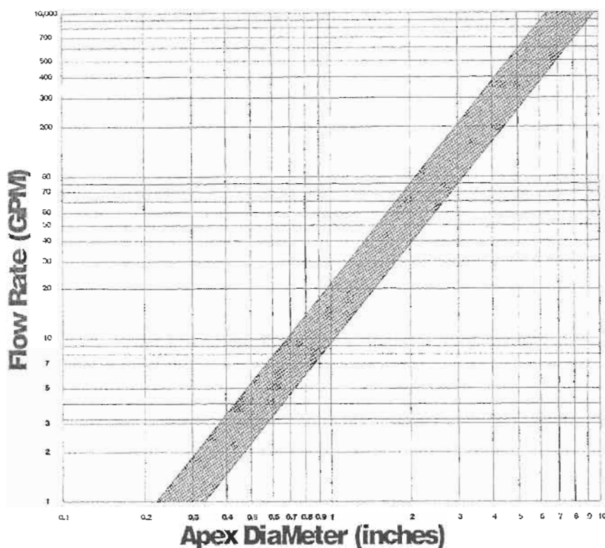
Figure 57. Apex capacity diameter vs flowrate, after Afterburn.
