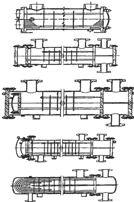
Figure 4. Common shell-and-tube exchanger configurations.
