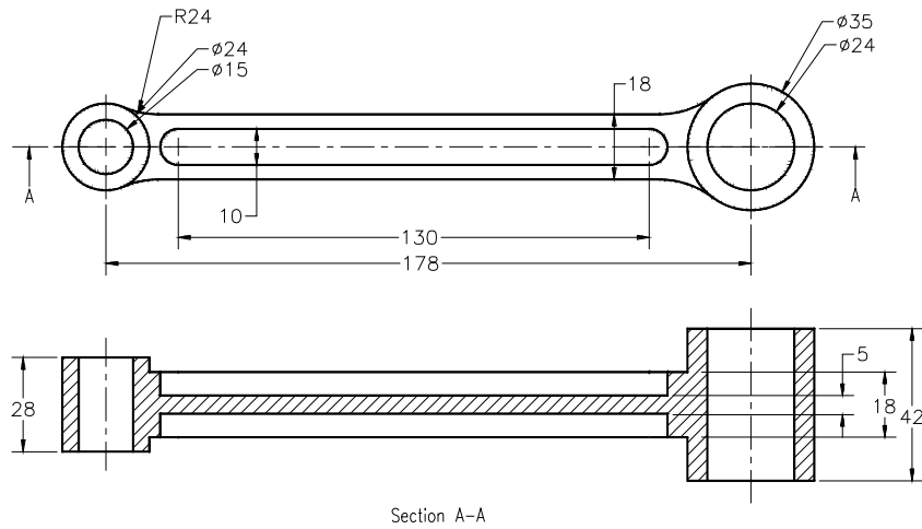
Figure 4 Views and dimensions of the Articulated Rod
