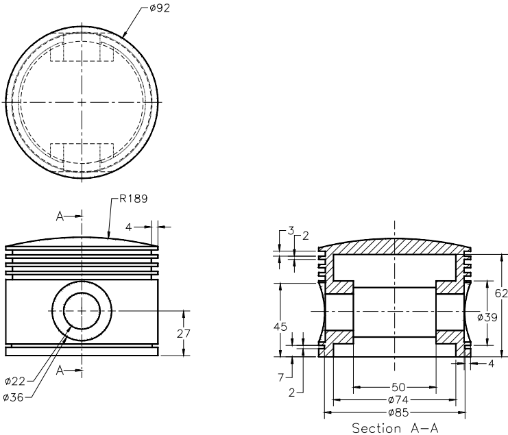
Figure 3 Views and dimensions of the Piston
