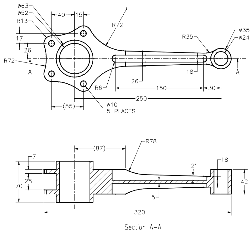
Figure 5 Views and dimensions of the Master Rod
